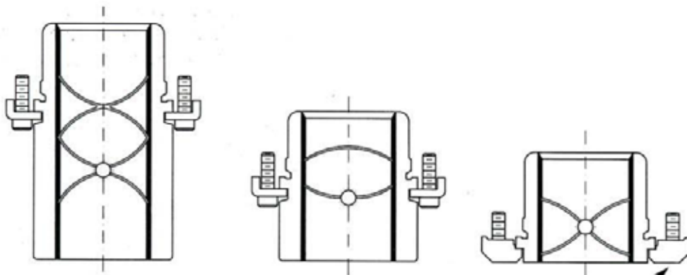
Brida estampada 5300 Stamped guide clamp
